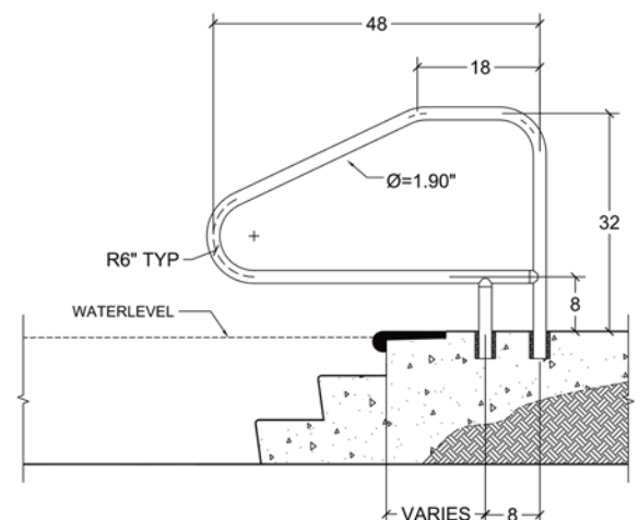
RETURN-TO-DECK HANDRAIL CBRTD-448 CROSS BRACED
