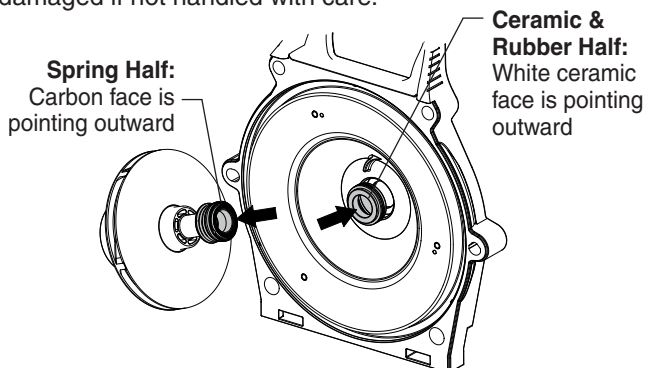
Mechanical Seal
