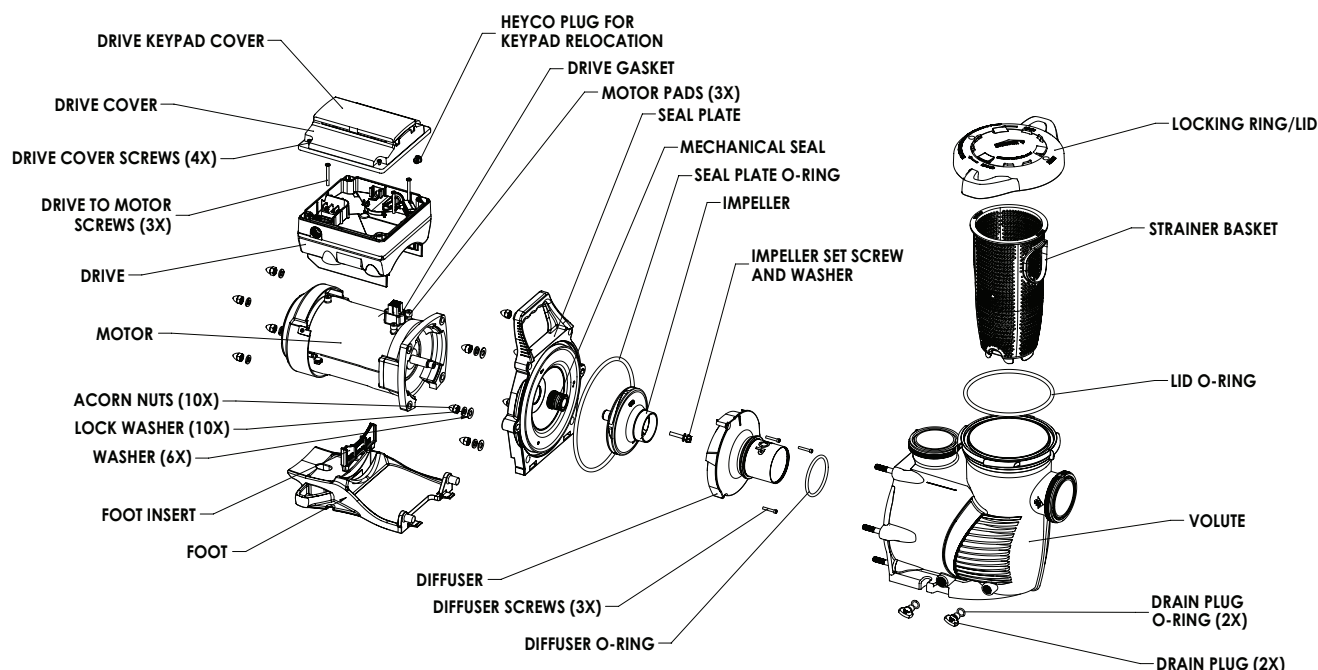
Pump Illustrated Parts View
