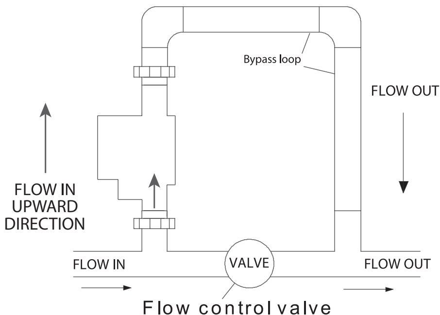
iChlor SCG System Loop Plumbing Diagram
