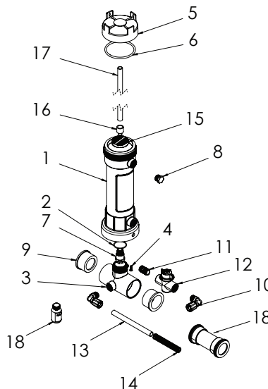
Part # CH100
